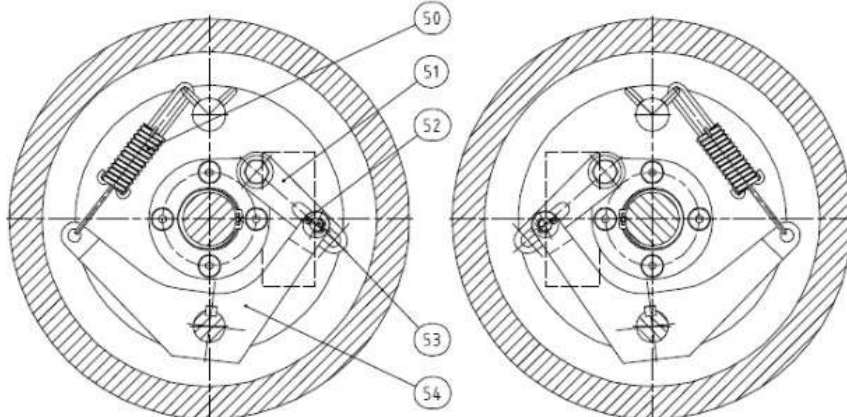
Section A-A (1:2)
